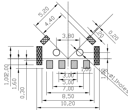
P. C. B. INSTALLATION DIAGRAM
