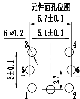
带灯轻触主要技术指标: Llluminated Tact Switch Main Specifications:
